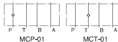
Graphic Symbols
