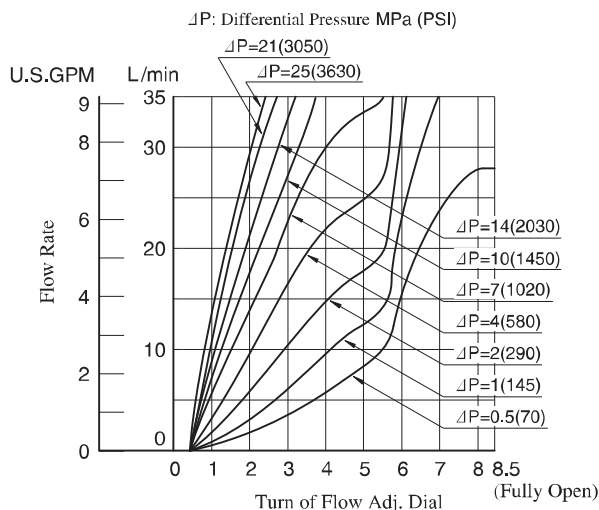
Metred Flow vs. Dial Position
