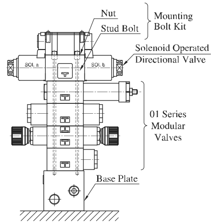
Stacking Example
