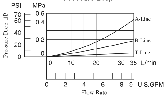
Pressure Drop
