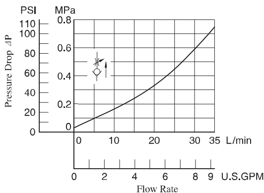
Pressure Drop at Throttle Fully Open
